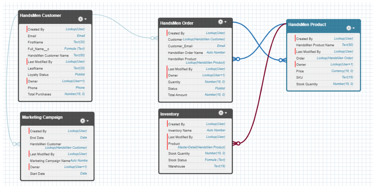
Figure 2 Schema Builder Data Model
