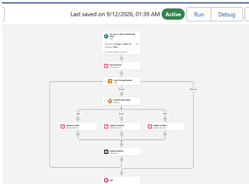
Figure 14 Loyalty Status Update Flow
